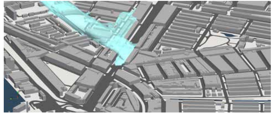
3D image of particulate matter dispersion at the Pleinweg, southwest wind
